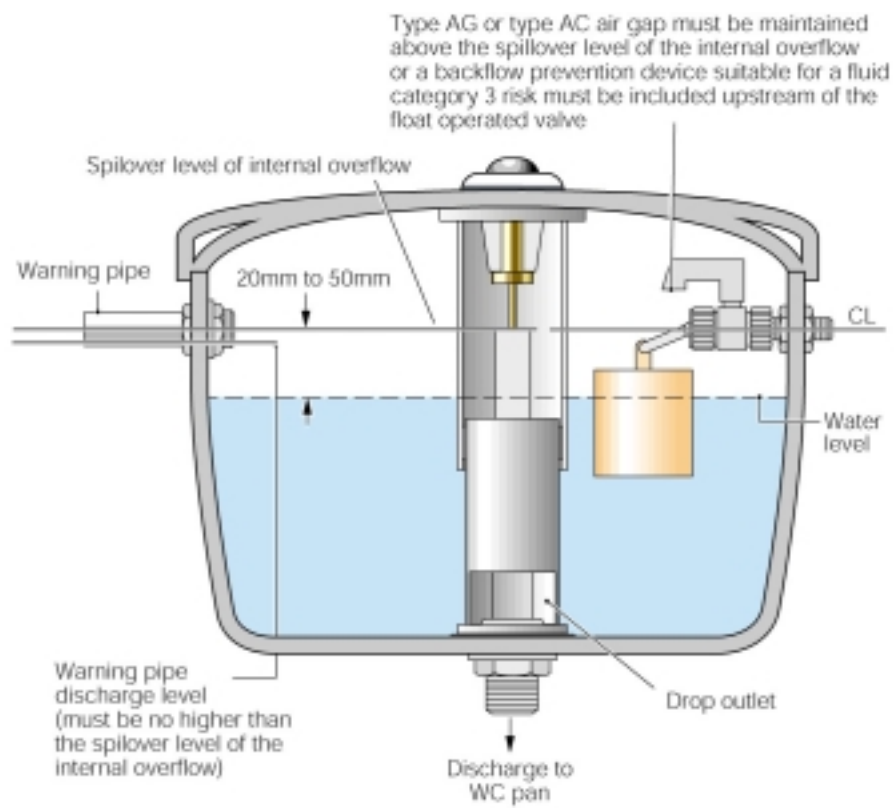
Figure 2 - WC Cistern with drop valve type flush.
